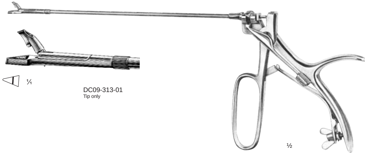
Schumacher DC09-313-00 Schumacher Biopsy Specimen Forceps with exchangeable tip
